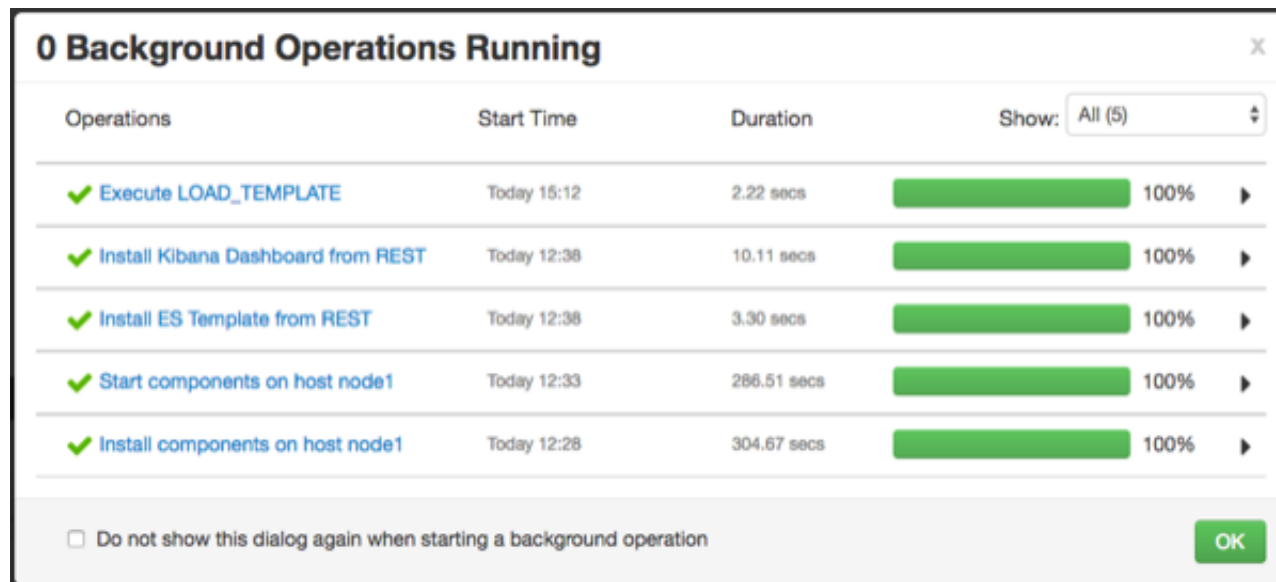
Figure 4.5. Ambari Background Operations
