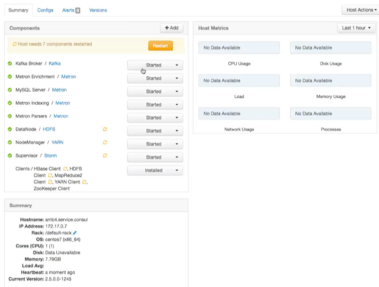
Figure 4.7. Components Window
