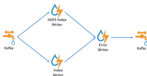
Figure 5.2. Indexing Architecture
