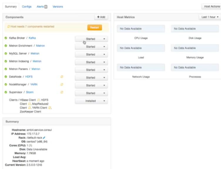
Figure 4.9. Components Window
