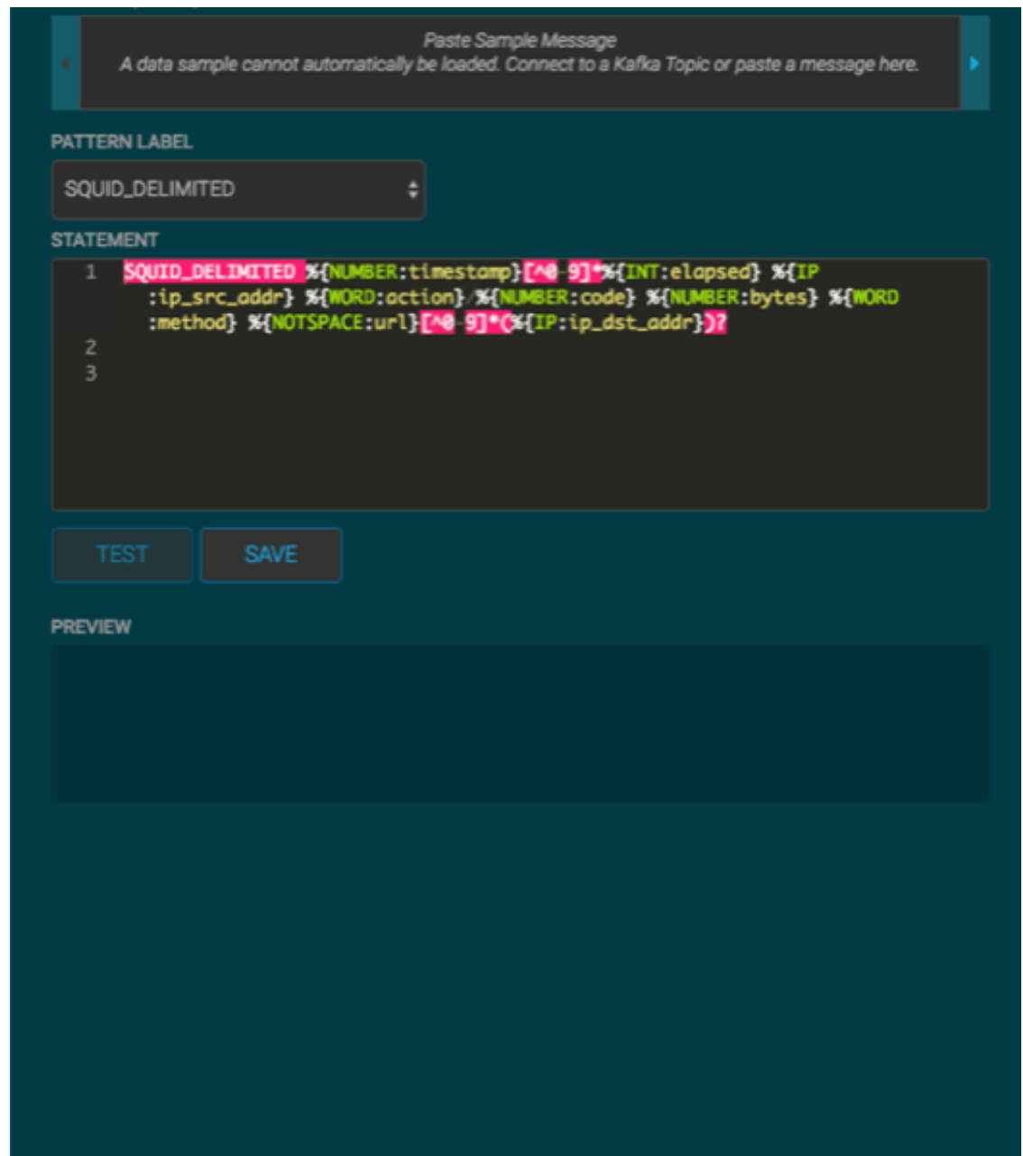
Figure 2.15. mm_grok_validator_squid_complete.png
