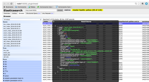
Figure 2.16. Elasticsearch
