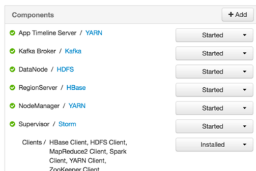
Figure 3.1. Ambari Component
