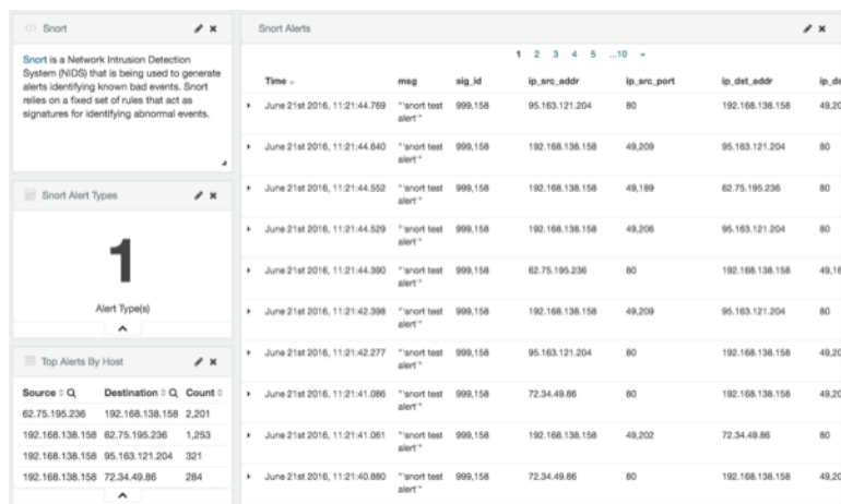
Figure 2.1. Dashboard-Snort Panel
