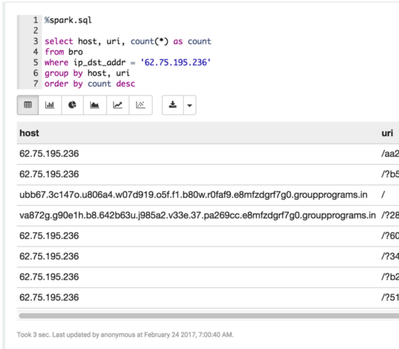
Figure 4.9. x-dosexyc Requests
