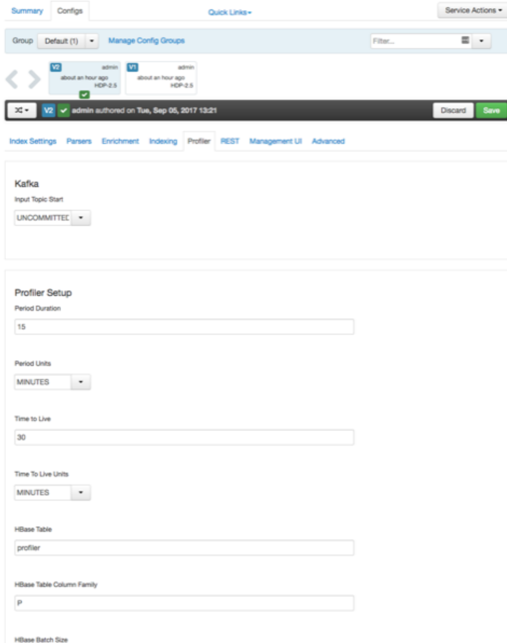
Figure 2.1. ambari_profiler_configs.png
