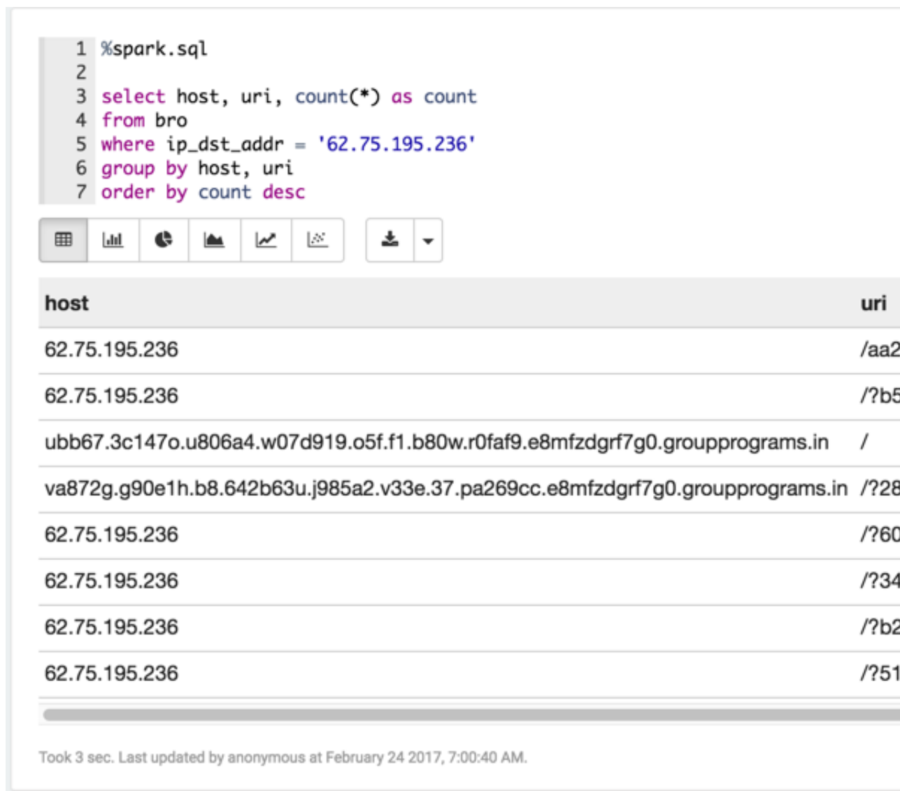
Figure 4.9. x-dosexcc Requests
