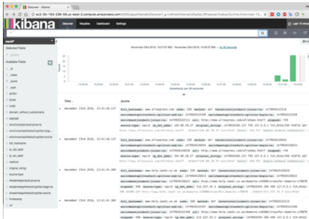
Figure 2.18. Discover Tab with Squid Elements
