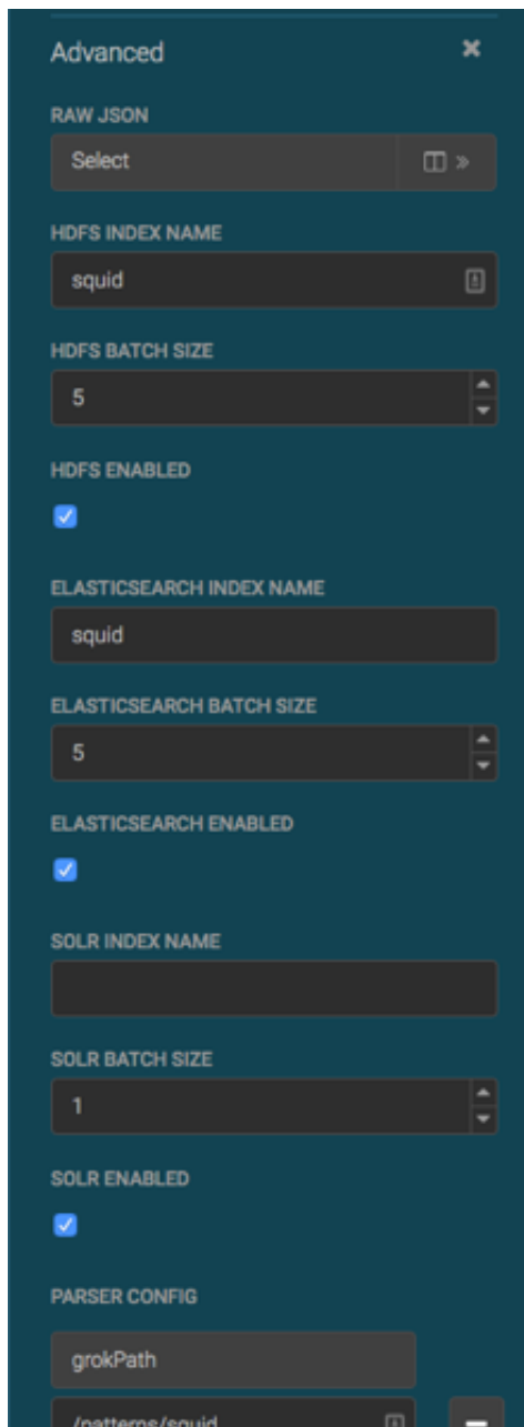
Figure 7.1. Management Module Advanced Panel
