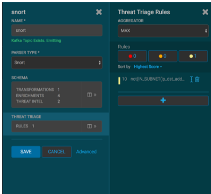
Figure 6.1. Threat Triage Rules Panel
