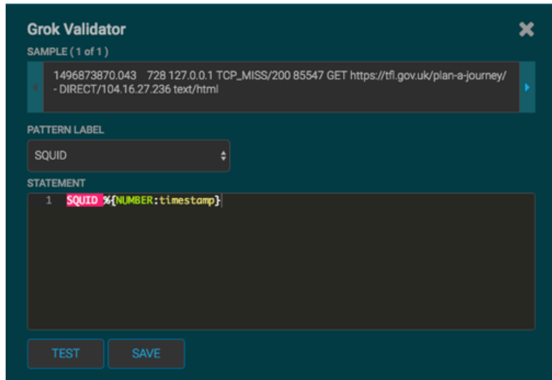
Figure 2.12. Grok Validator Panel with Statement Information
