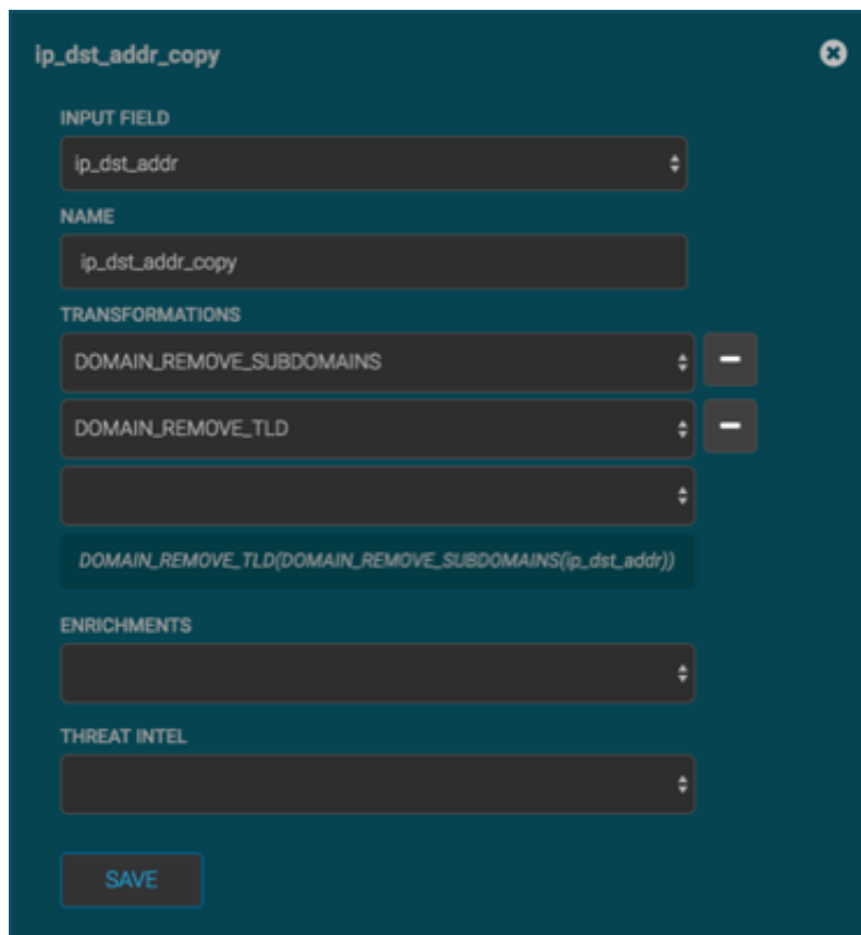
Figure 3.3. Populated Schema Information Panel
