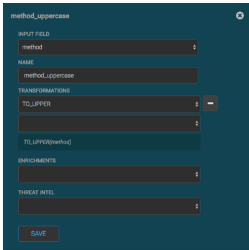
Figure 4.2. Populated New Schema Information Panel
