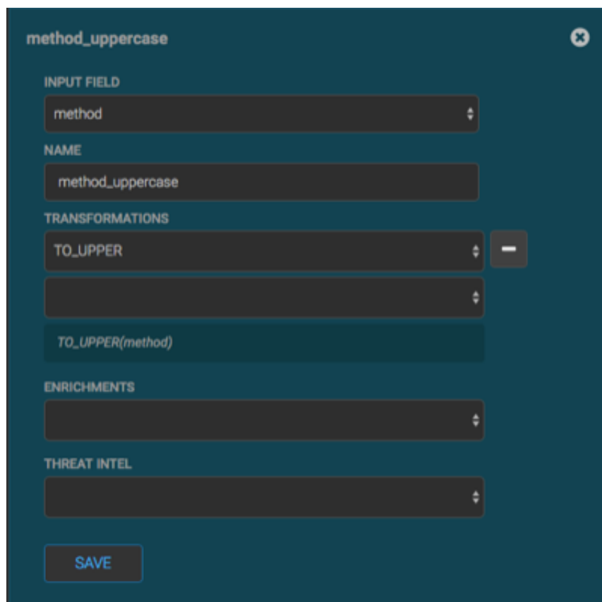
Figure 5.2. Populated New Schema Information Panel
