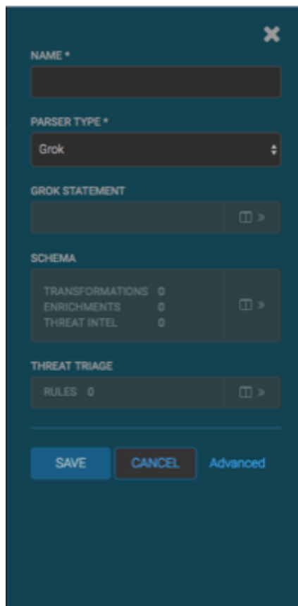
Figure 2.10. New Sensor Panel
