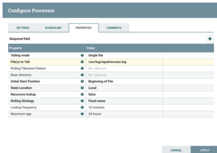
Figure 2.4. Configure Processor Dialog Box Properties Tab
