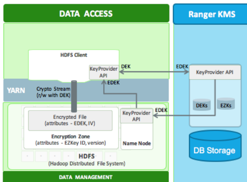
Figure 13.1. HDFS Encryption Components
