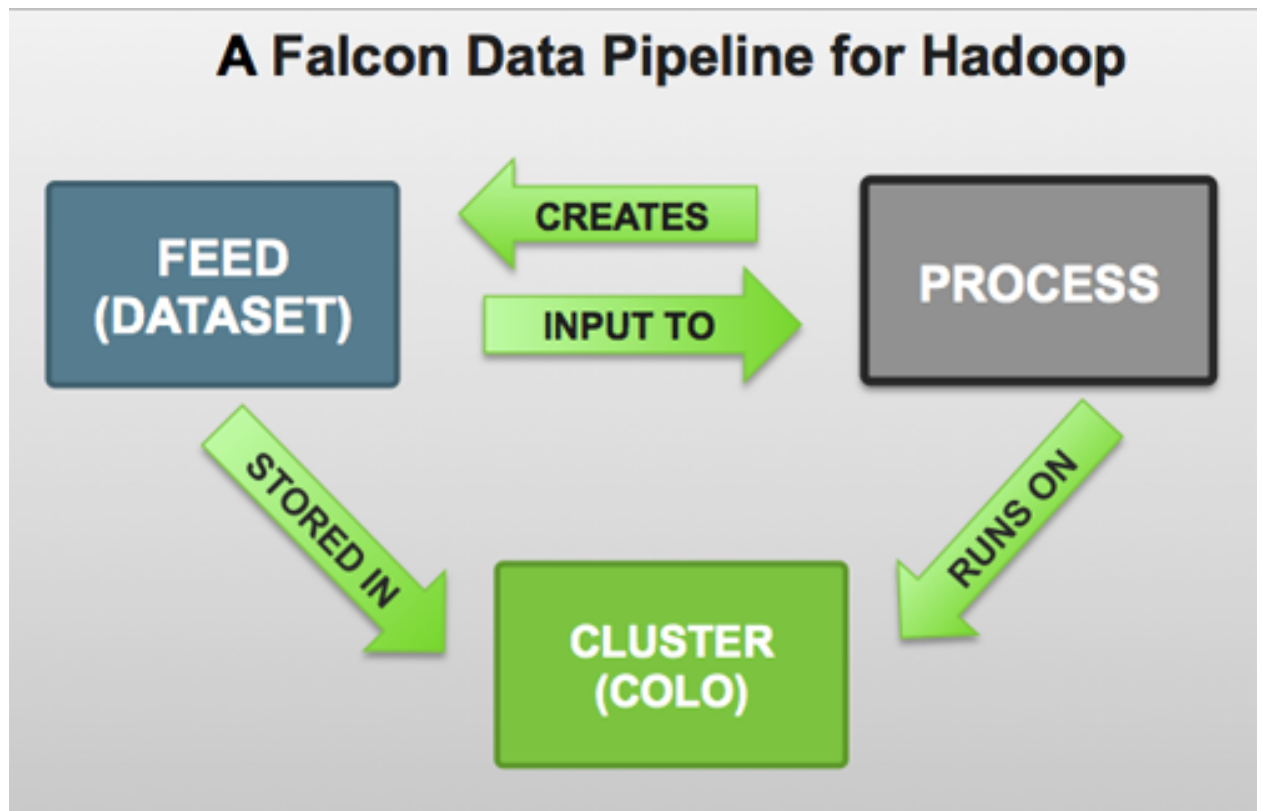
Figure 2.2. Data Pipeline
