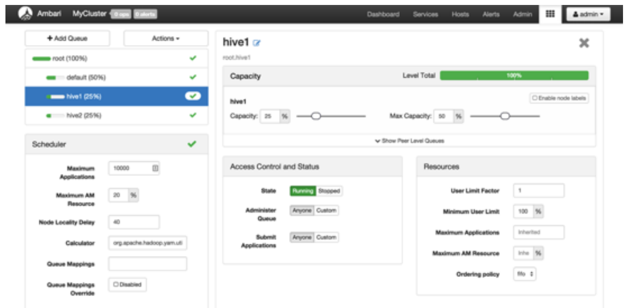
Figure 4.3. Ambari Capacity Scheduler View
