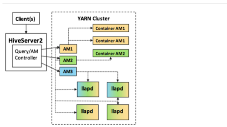
Figure 2.1. LLAP on Your Cluster
