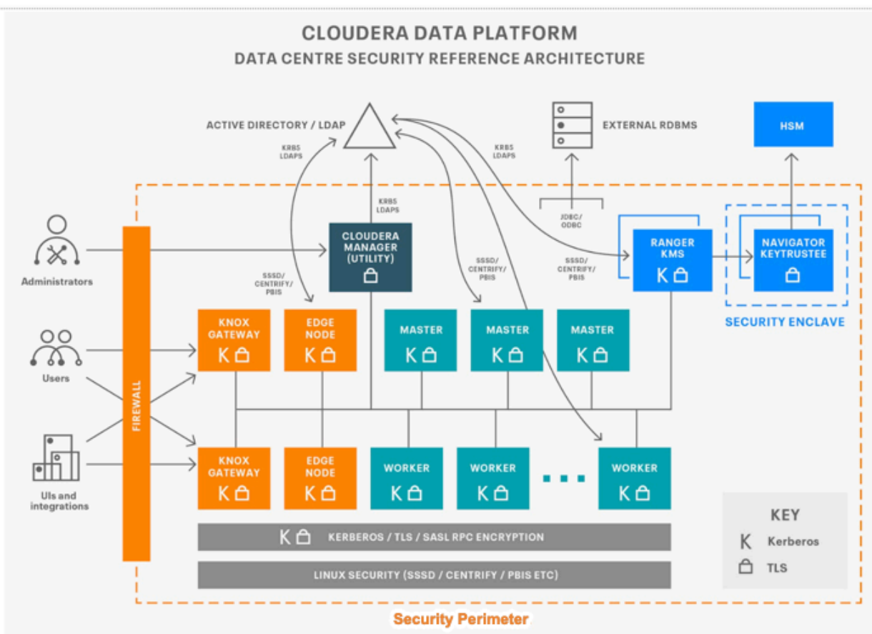
Figure 3: CDP Private Cloud Security Architecture
