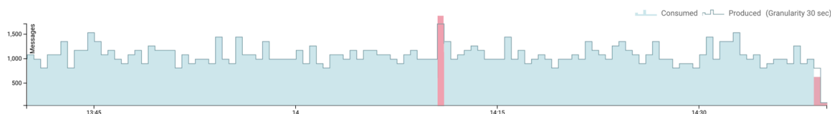
Messages Consumed
