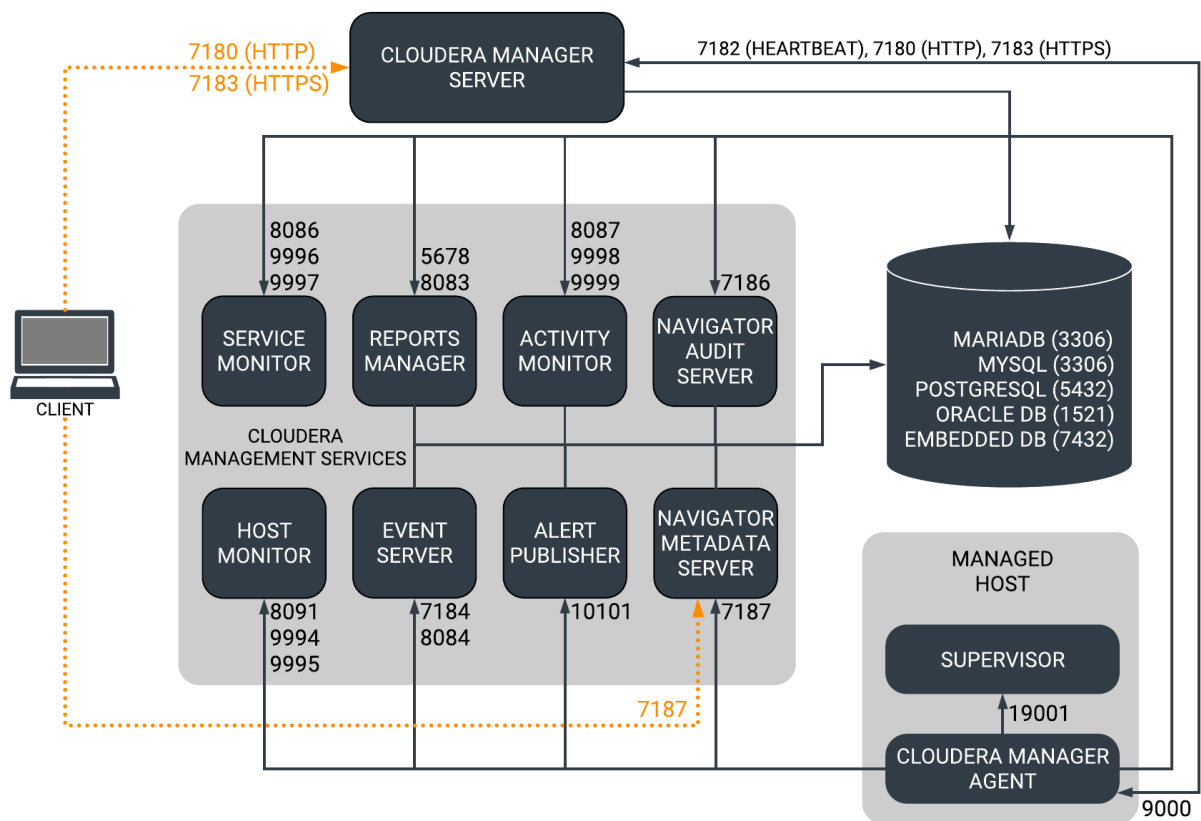
Figure 1: Ports Used by Cloudera Manager
