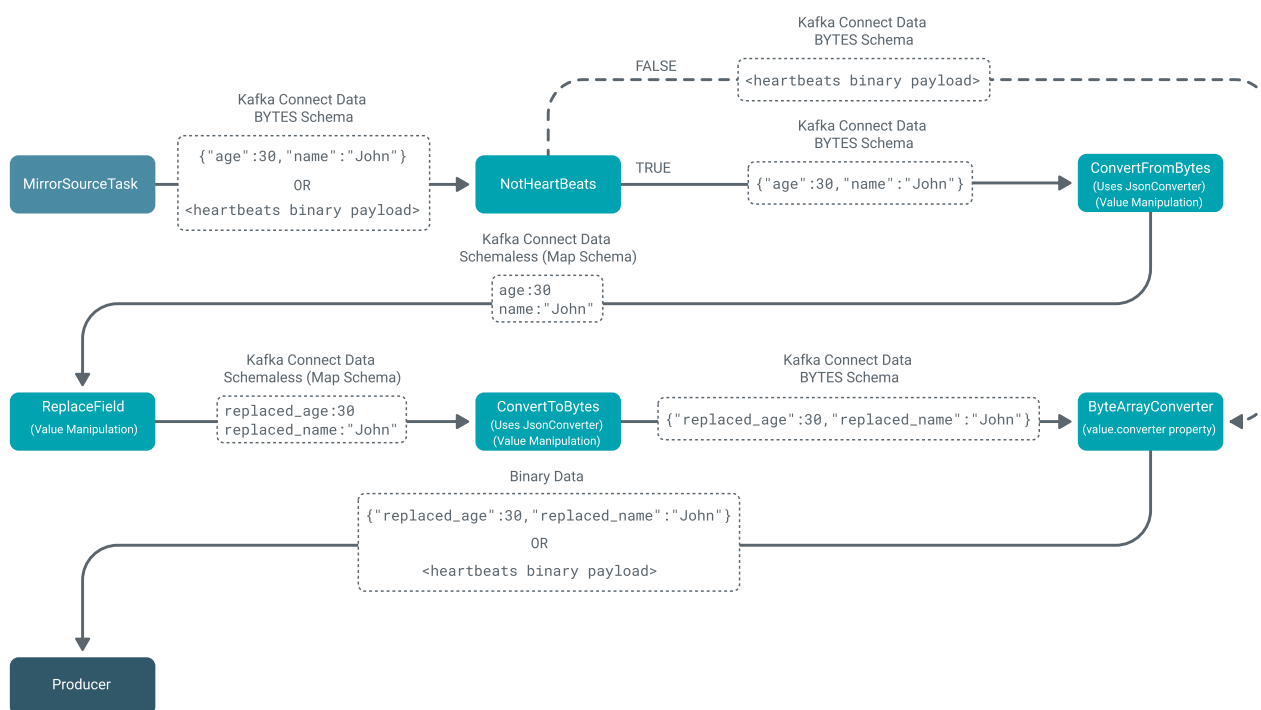
Figure 5: Value conversion with a predicate that filters heartbeat records
