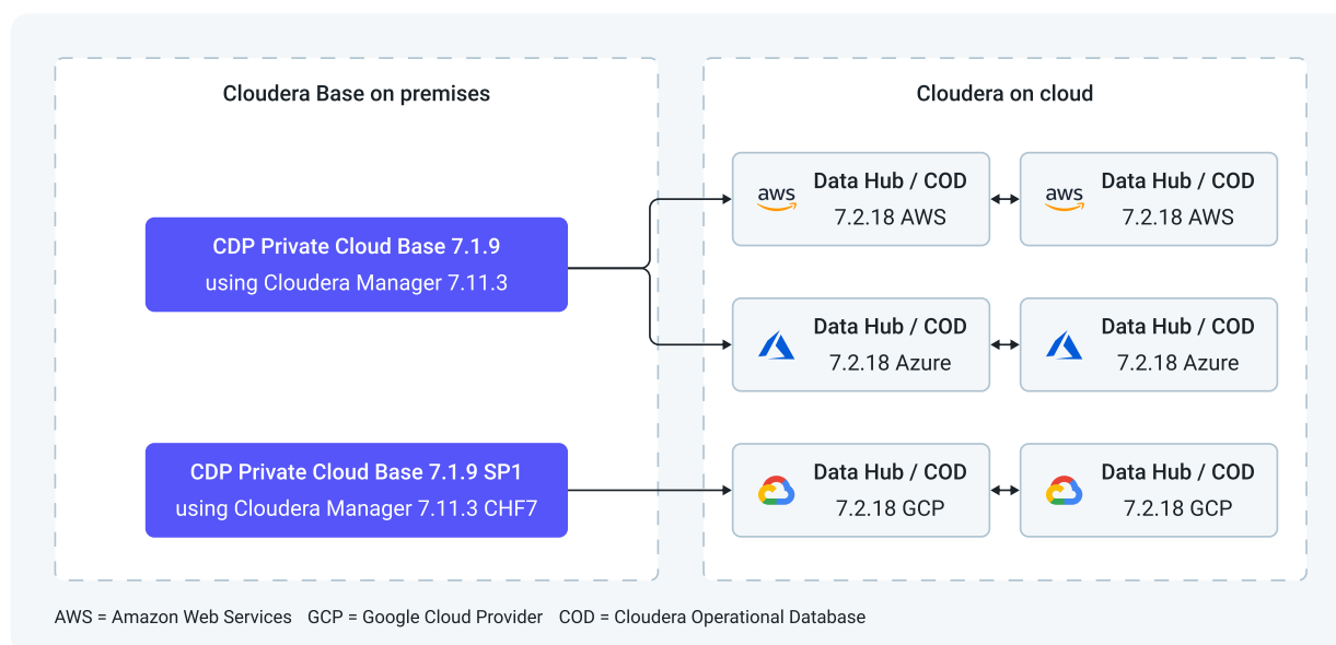
Figure 8: Lowest supported versions for HBase replication policies
