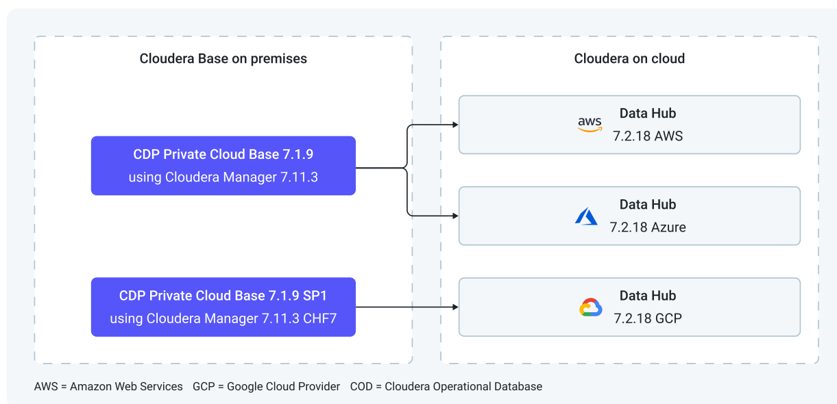
Figure 6: Lowest supported versions for Hive replication policies
