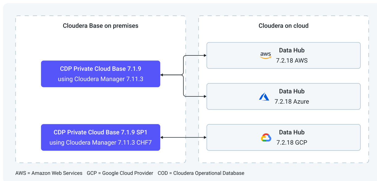
Figure 4: Lowest supported versions for HDFS replication policies
