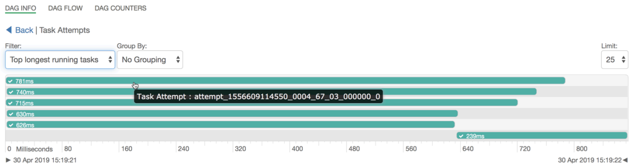
Figure 4: DAG info: Viewing task attempt
