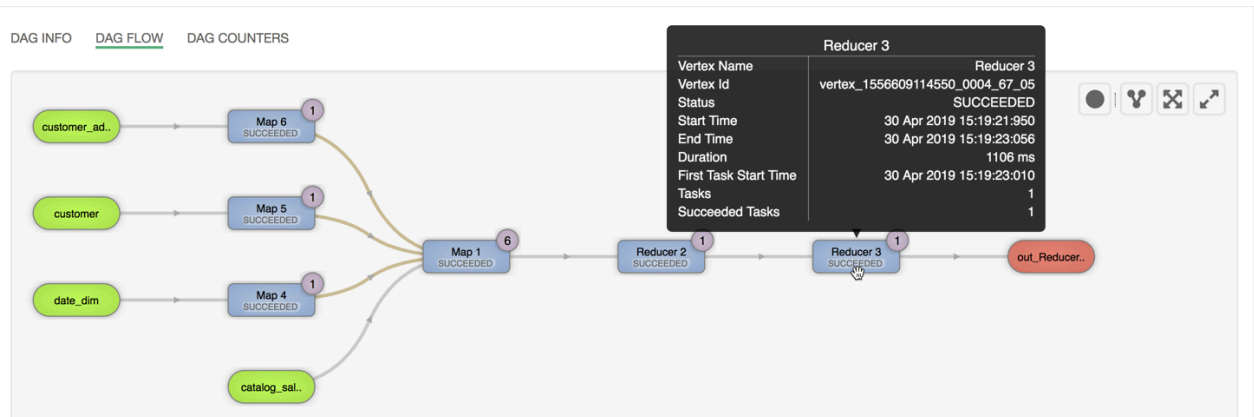
Figure 5: DAG flowchart
