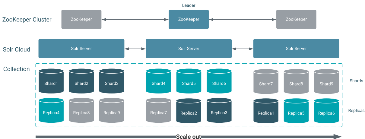
Figure 1: Solr scaling
