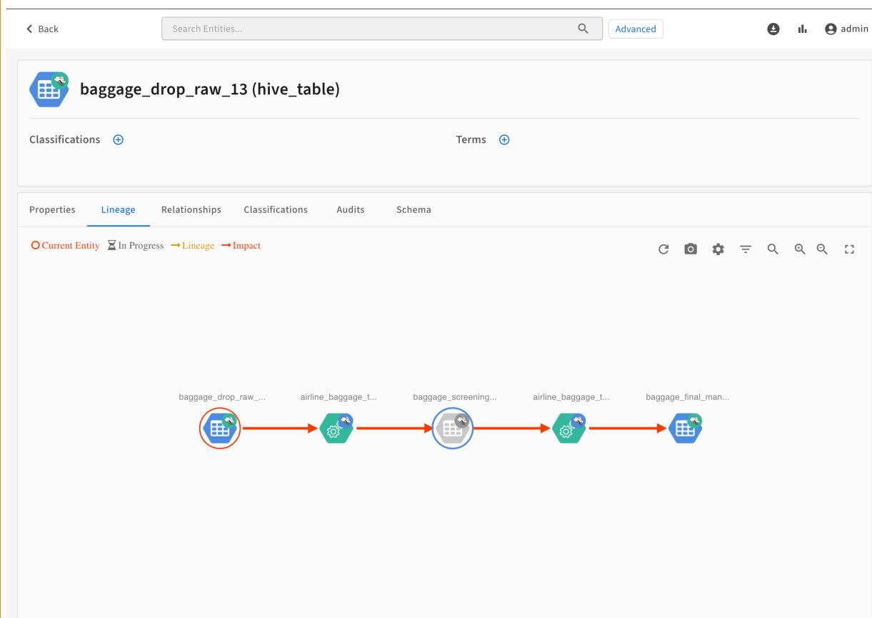
Figure 2: Sparse graph with deleted Hive table
