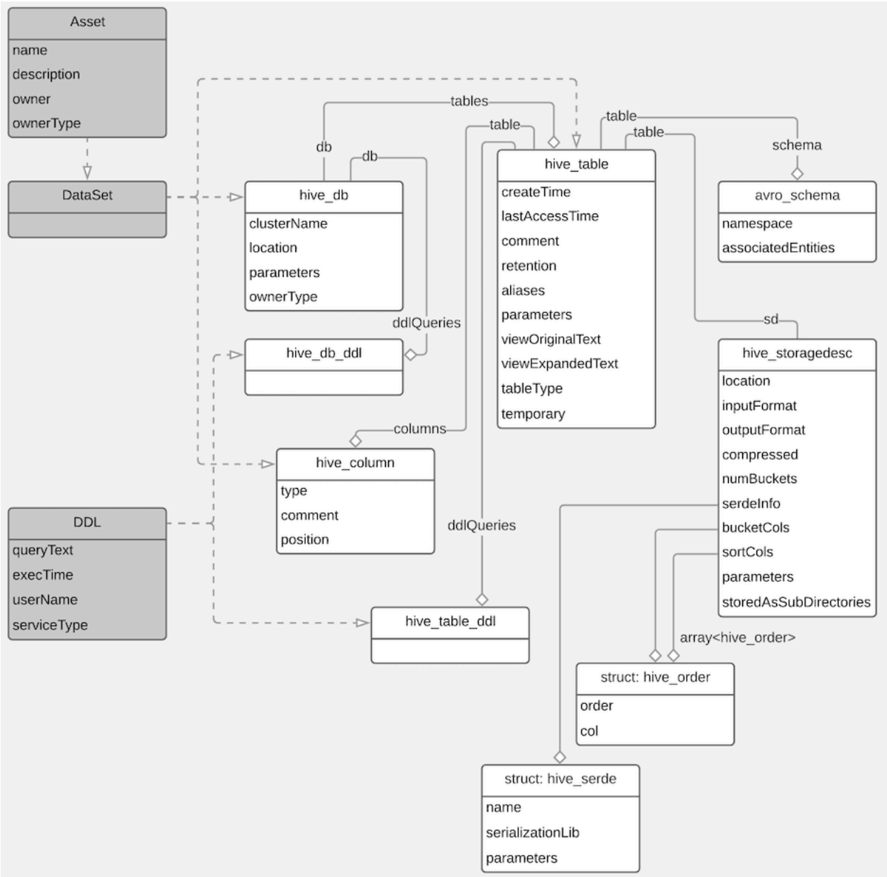
Figure 12: Atlas Entity Types for HiveServer Processes
